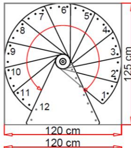
12 Stufen (Standard) 12 steps (standard)
