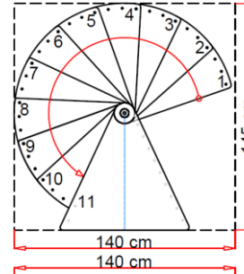
11 Stufen (Standard-1) 11 steps (standard-1)
